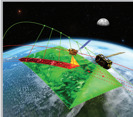
CLARREO Pathfinder Calibration and Inter-Calibration Concepts: CLARREO Pathfinder has two primary objectives to demonstrate essential measurement technologies on orbit: 1) (top) calibrate the instrument using stable, well-known sources: the Sun and the Moon and 2) (bottom) transfer that calibration to other instruments that cross its path.
